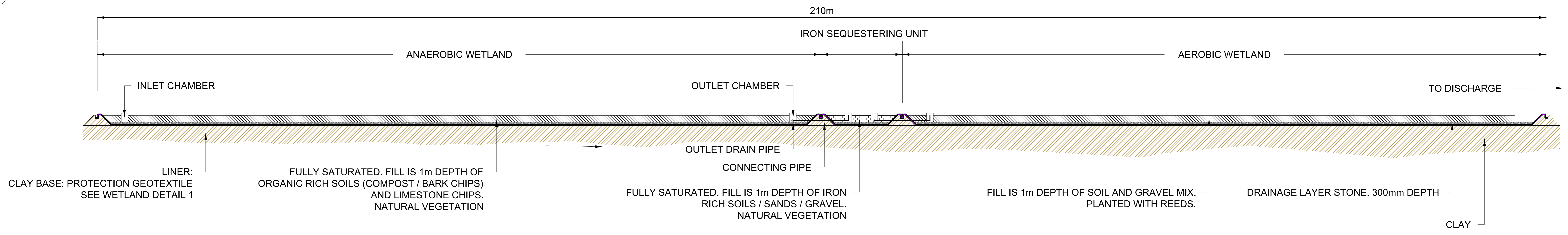
INDICATIVE PROPOSED TREATMENT LAYOUT - SECTION A-A' VIEW
