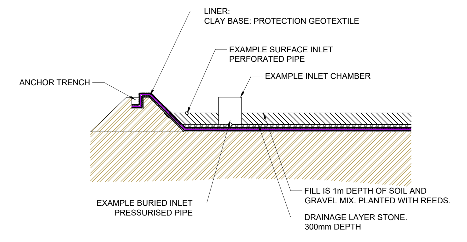
WETLAND DETAIL 1 SCALE 1:200
