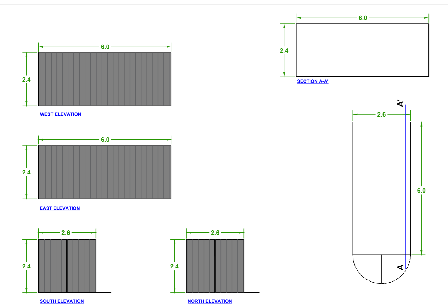
6 x 2.6m ISO CONTAINER SCALE 1:100
