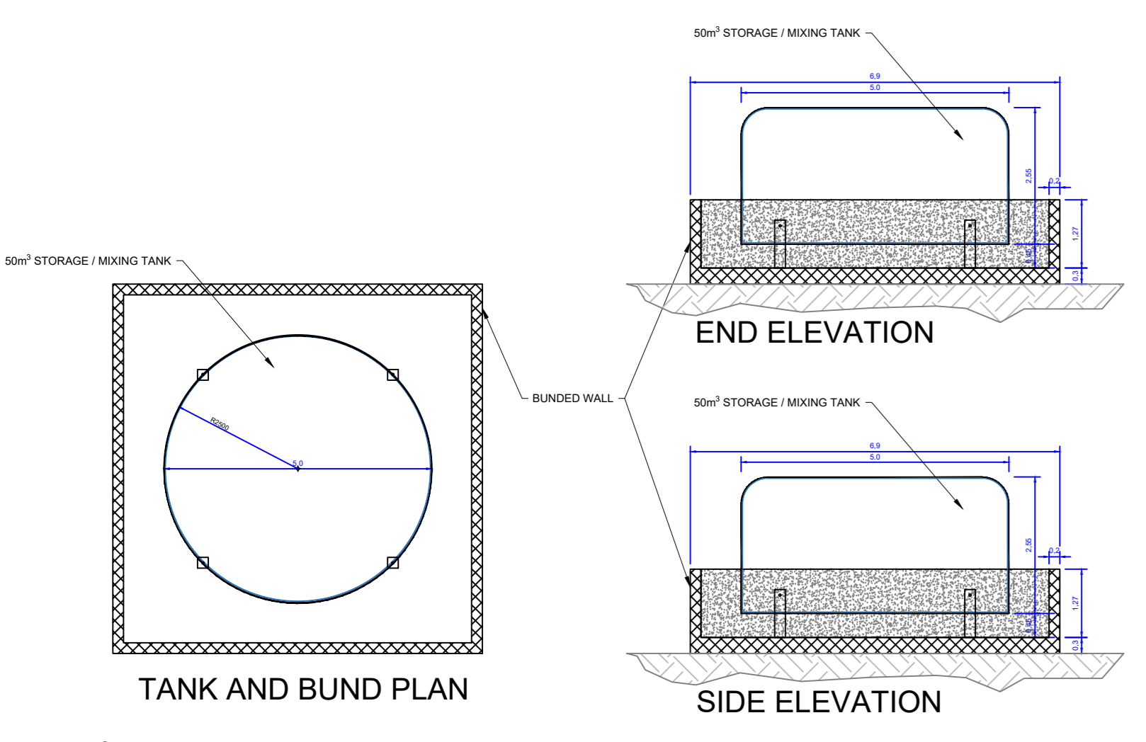
50m³ STORAGE / MIXING TANK SCALE 1:100
