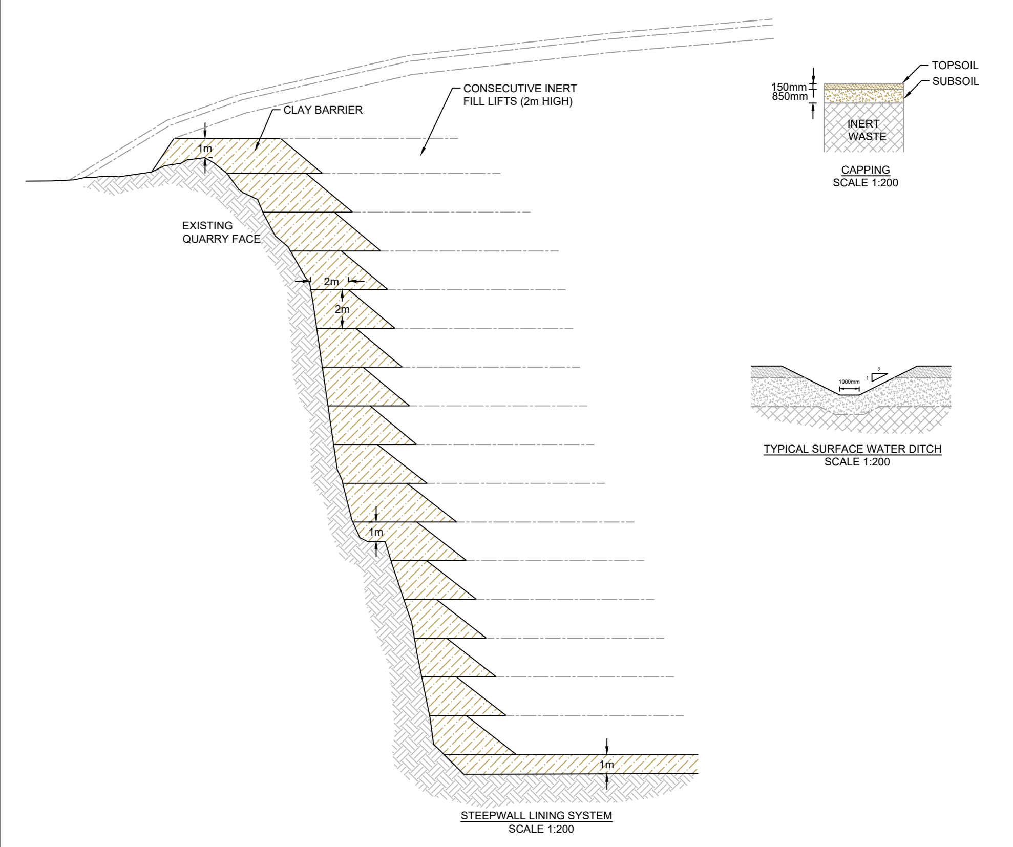
LANDFILL LINEAR DETAIL 1 SCALE 1:200
